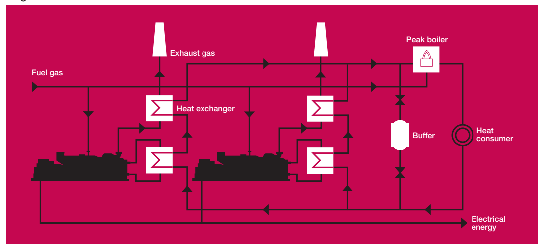
Cogeneration Schematic
