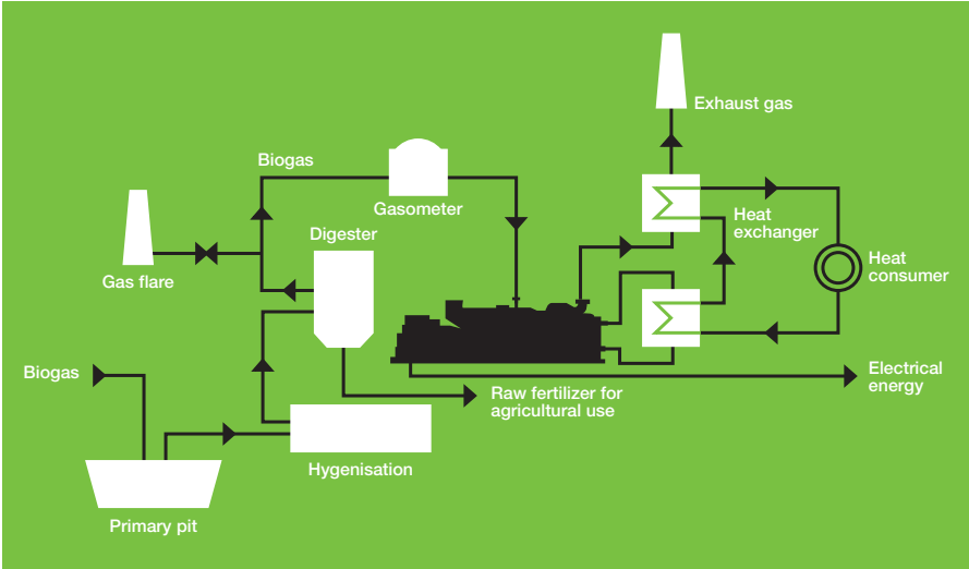
Agricultural Biogas Schematic
