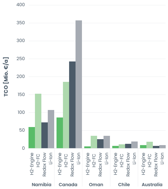
Figure 18: Capital expenditures (CAPEX) and total cost of ownership (TCO) for the different backup solutions
