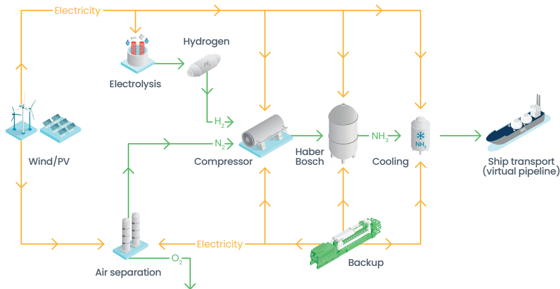
Figure 3: Basic setup of a green ammonia production facility
