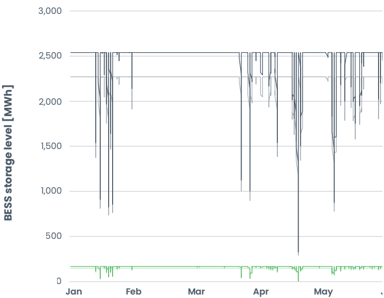
Figure 16: Required storage capacity for BESS-backup solution – case study Namibia
