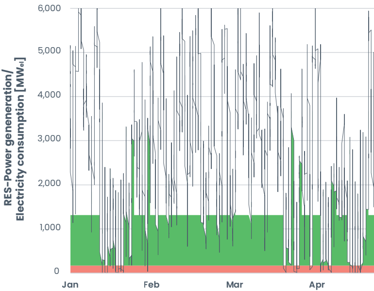
Figure 12: Electricity consumption for H 2 production and Haber Bosch process (including air separation, compression, reactor and ammonia cooling) – case study Namibia
