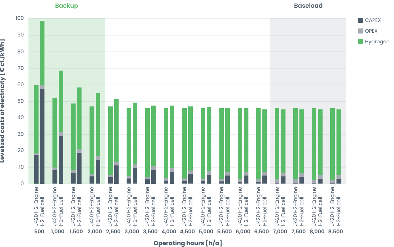
Figure 9: Levelized cost of electricity (LCOE) for H2-Engines and H2-Fuel cells
