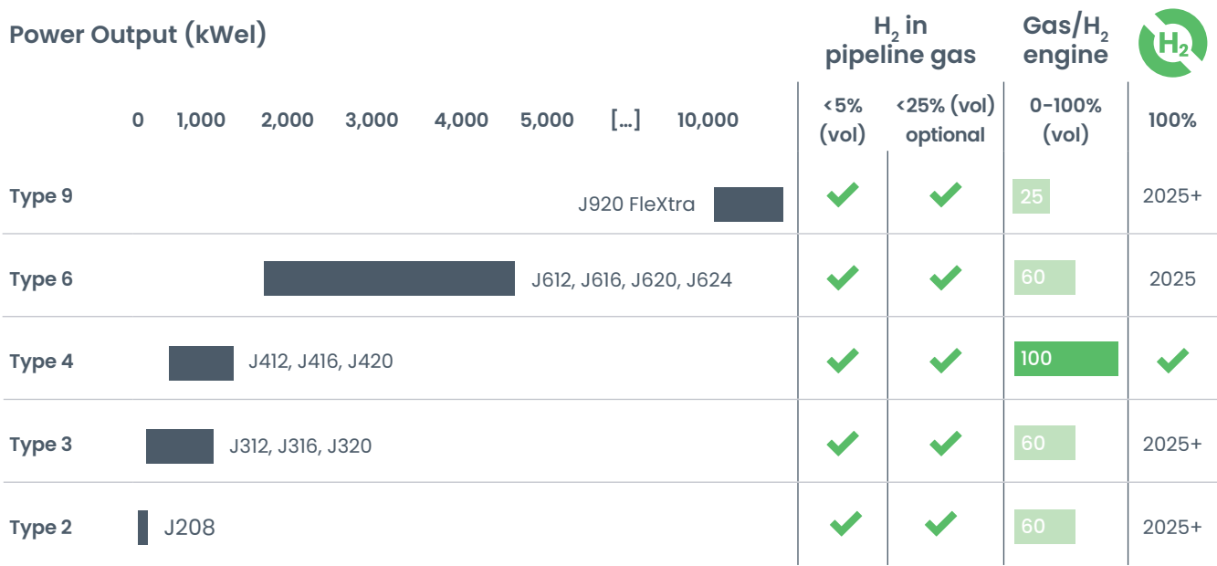
Figure 6: Jenbacher “Ready for H 2 ” product portfolio
