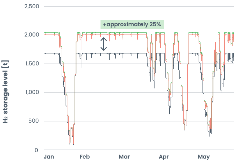
Figure 15: Required additional H 2 storage capacities for H 2 -based backup power systems – case study Namibia
