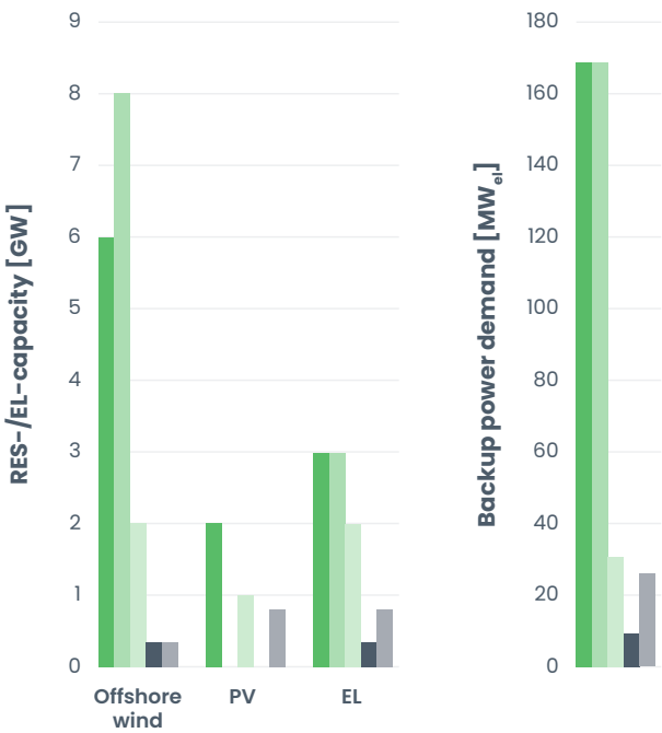
Figure 13: Available RES/EL-Capacity (left), required peak backup power (middle) and monthly demand for backup power (right)
