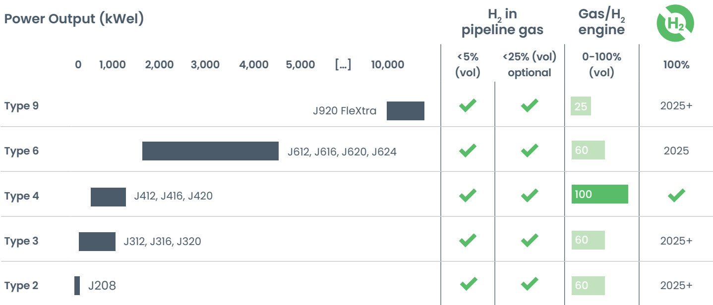
Figure 8: Jenbacher “Ready for H 2 ” product portfolio
