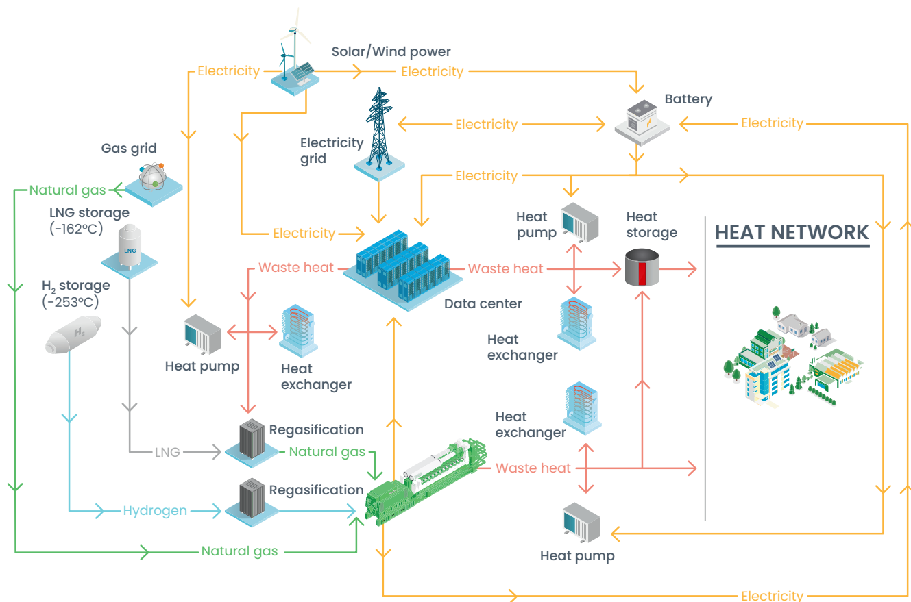
Figure 11: Regionally integrated decarbonization of data centers
