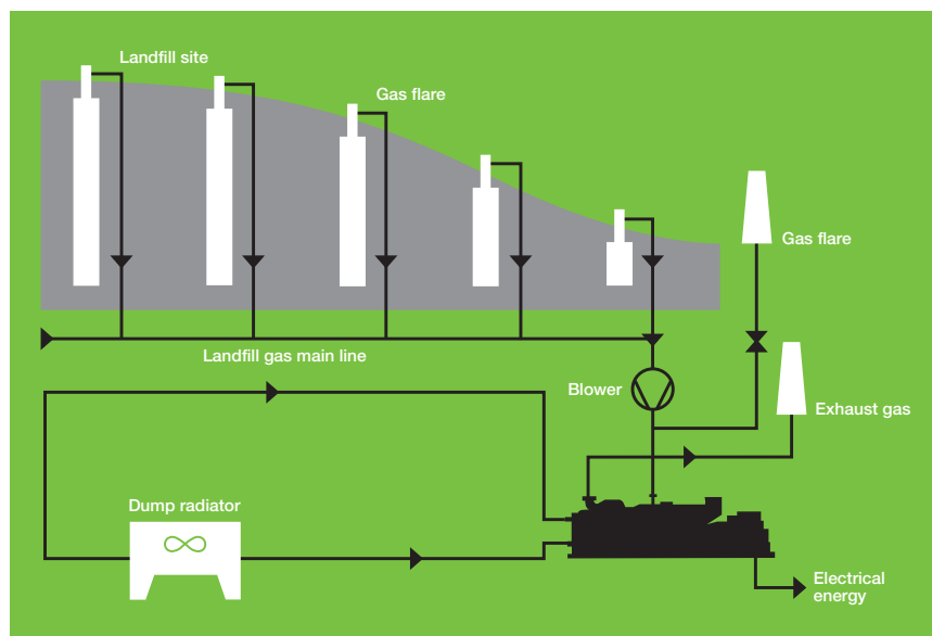
Landfill Gas Schematic
